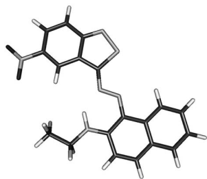
Figure 1. Structure of azo compound 2b calculated by using the B3LYP/TZVP method.
