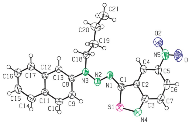
Figure 3. ORTEP view of one of two independent molecules of triazene 1c showing the thermal ellipsoids at 50% probability; selected bond lengths [Å] and angles [°]: S1–N4 1.651(3), S1–C1 1.706(3), S1'–N4' 1.644(3), S1'–C1' 1.708(4), N3–N2 1.314(4), N3–C8 1.419(4), N3–C18 1.480(4), N3'–N2' 1.320(4), N3'–C8' 1.429(4), N3'–C18' 1.473(4), N1–N2 1.295(4), N1–C1 1.372(4), N2'–N1' 1.284(4), N1'–C1' 1.363(4), C3–N4 1.325(5), N5–O2 1.200(5), N5–O1 1.213(4), N5–C5 1.473(5), N4'–C3' 1.336(5), N5'–O2' 1.212(6), N5'–O1' 1.230(5), N5'–1.477(6); N4–S1–C1 97.12(16), N4'–S1'–C1' 96.95(17), N2–N3–C8 116.1(3), N2–N3–C18 121.2(2), C8–N3–C18 122.7(3), N2'–N3'–C8' 115.7(3), N2'–N3'–C18' 121.1(3), C8'–N3'–C18' 123.1(3), N2–N1–C1 109.7(3), N1'–N2'–N3' 114.3(3), N2'–N1'–C1' 110.7(3), N1–N2–N3 114.8(3), C13–C8–N3 120.5(3), C9–C8–N3 119.3(3), N4–C3–C7 123.9(3), N4–C3–C2 117.5(3), C3–N4–S1 108.1(2), C13'–C8'–N3' 120.5(3), C9'–C8'–N3' 119.7(3), N1'–C2'–124.5(3), N1'–C1'–S1' 128.3(3), C2'–C1'–S1' 107.2(3), C20–C19–C18–113.6(3), N3–C18–C19 111.9(3), N3'–C18'–C19' 112.0(3), O2–N5–O1 124.5(4), O2–N5–C5 118.7(3), O1–N5–C5 116.8(4), N1–C1–C2 124.4(3), N1–C1–S1 127.7(3), C2–C1–S1 107.9(2), C4–C5–N5 118.3(3), C6–C5–N5 118.6(3), C3'–N4'–S1' 108.8(3), C10'–C9'–C8' 120.3(3), N4'–C3'–C2' 116.1(3), N4'–C3'–C7' 124.6(4), C2'–C7'–119.2(4), O2'–N5'–O1' 123.7(5), O2'–N5'–C5' 118.8(4), O1'–N5'–C5' 117.5(5), C4'–C5'–N5' 117.6(4), C6'–C5'–N5' 118.9(4).
