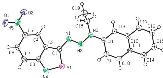
Figure 2. ORTEP view of triazene 1b showing the thermal ellipsoids at 50% probability; selected bond lengths [Å] and angles [°]: S1–N4 1.646(3), S1–C1 1.707(3), N1–1.279(4), N1–C1 1.379(4), N4–C3 1.338(4), N3–N2 1.323(4), N3–C8 1.412(4), N3–C18 1.483(4), O1–N5 1.214(4), N5–O2 1.224(4), N5–1.457(4); N4–S1–C1 96.50(16), N2–N1–C1 111.0(3), C3–N4–S1 108.9(2), N2–N3–C8 116.0(3), N2–N3–C18 120.0(3), C8–N3–C18 123.8(3), N1–N2–N3 114.4(3), N1–C1–C2 124.1(3), N1–S1–127.8(2), C2–C1–S1 108.1(3), O1–N5–O2 122.8(3), O1–N5–C5 119.0(3), O2–N5–C5 118.2(3), C4–C5–N5 118.6(3), C6–C5–N5 118.3(3), C13–C8–N3 120.2(3), N3–C8–C9 120.1(3), N4–C3–C7 124.5(3), N4–C3–C2 115.9(3), N3–C18–C19 111.9(3).
